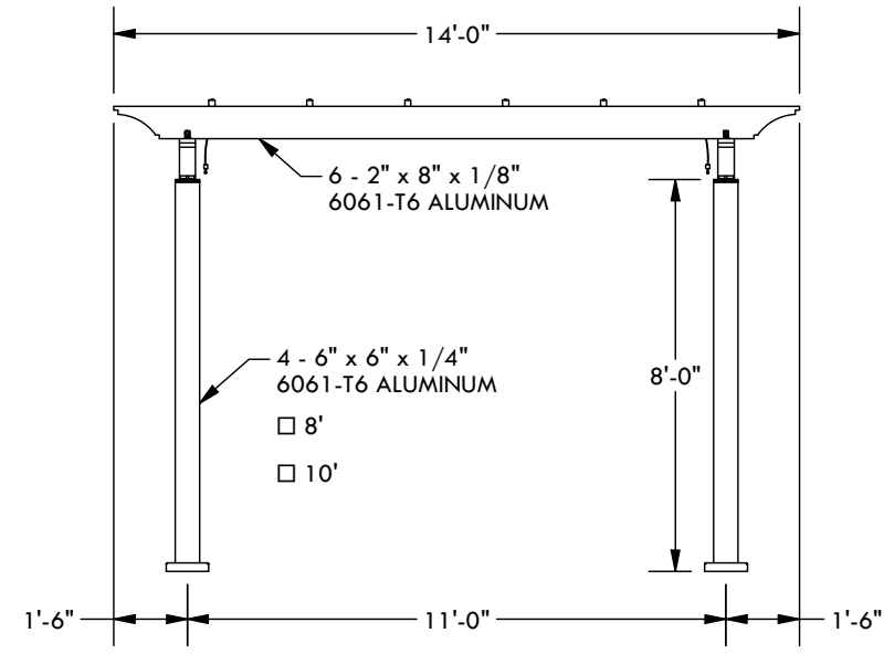
PROJECTION ELEVATION
