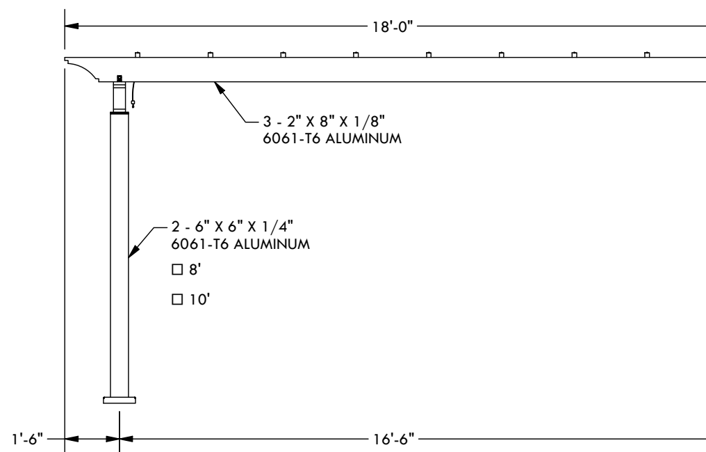
PROJECTION ELEVATION
