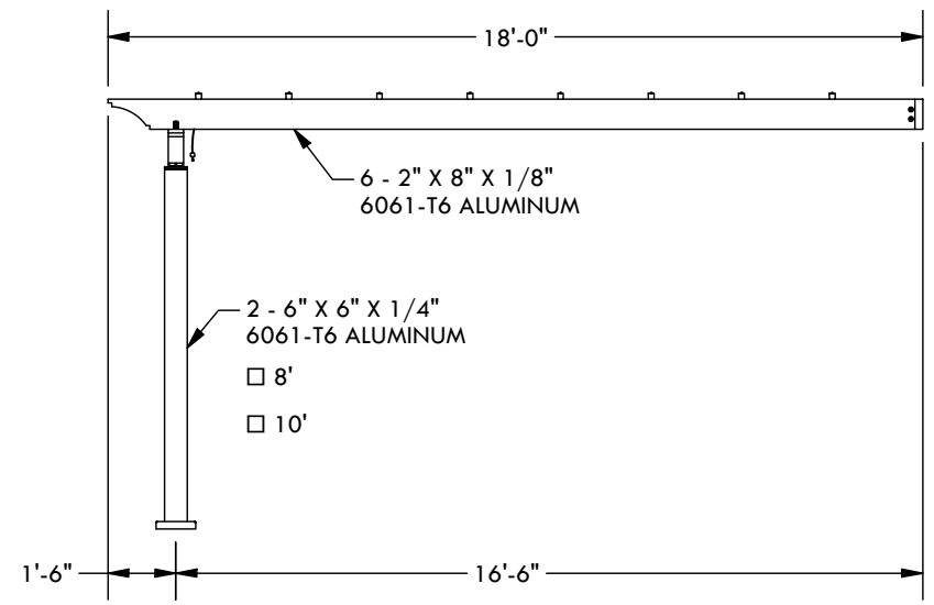
PROJECTION ELEVATION
