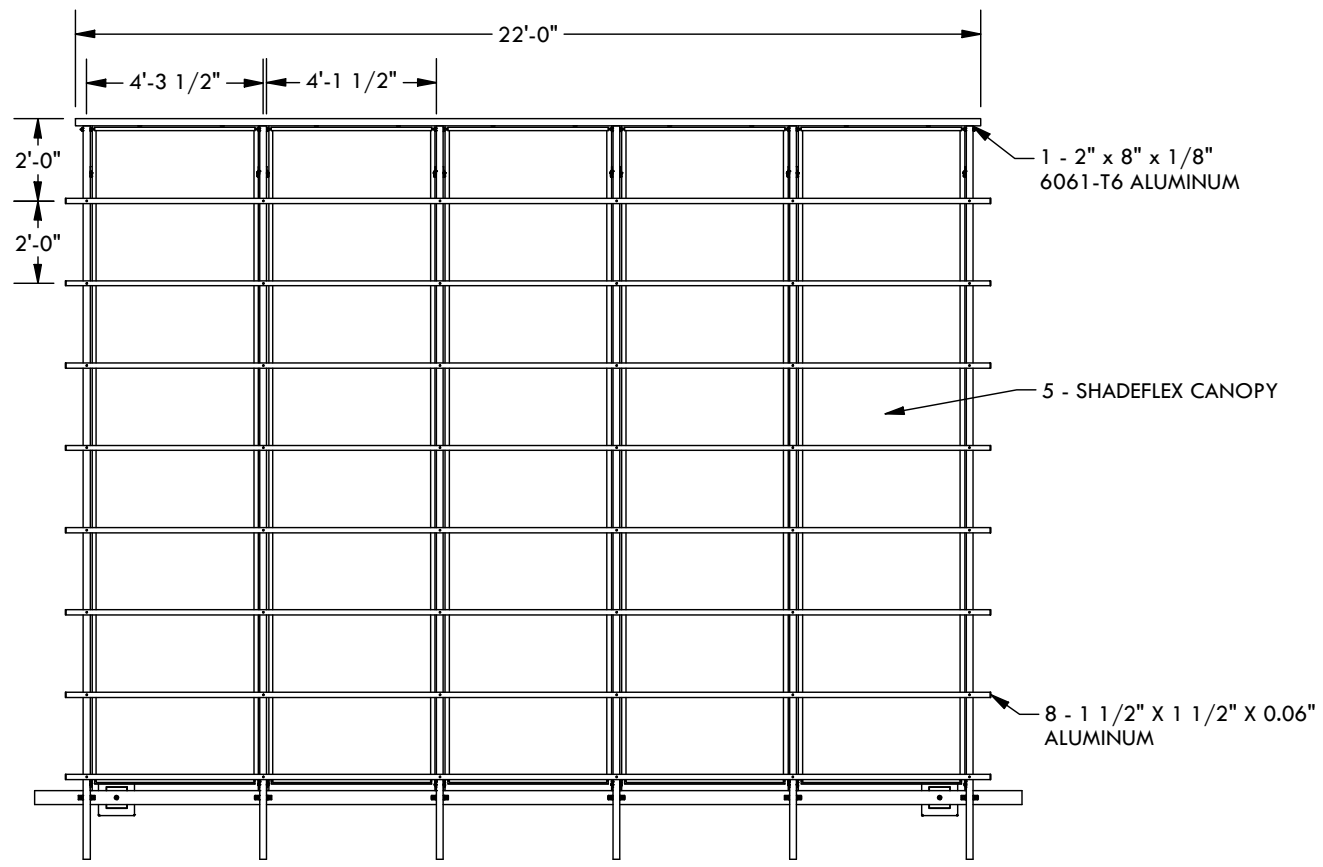
PLAN VIEW
