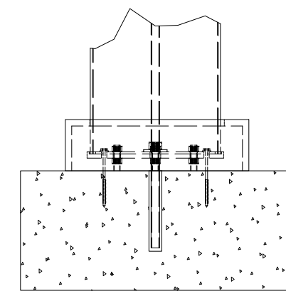
CONCRETE MOUNT
