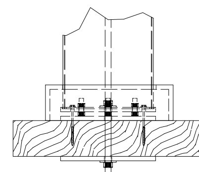
FRAMING MOUNT
