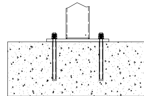
CONCRETE MOUNT
