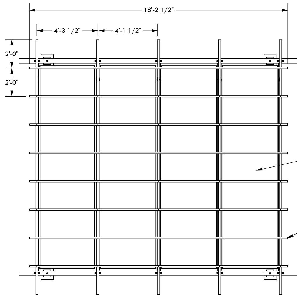
PLAN VIEW
