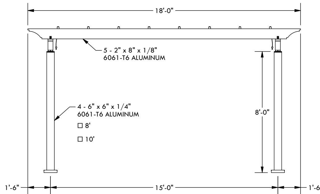
PROJECTION ELEVATION
