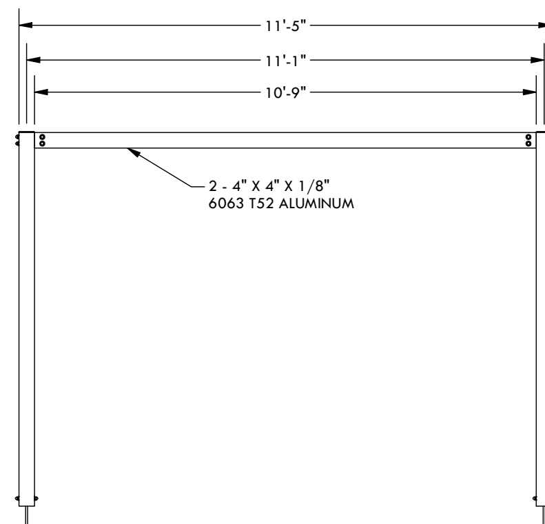
PROJECTION ELEVATION
