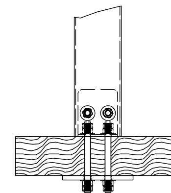
FRAMING MOUNT
