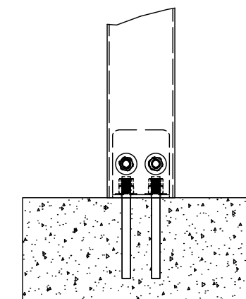
CONCRETE MOUNT
