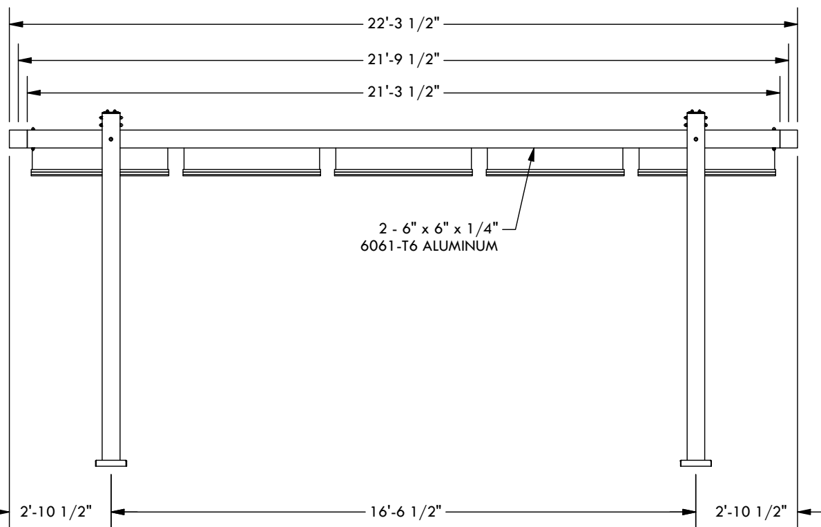
PROJECTION ELEVATION
