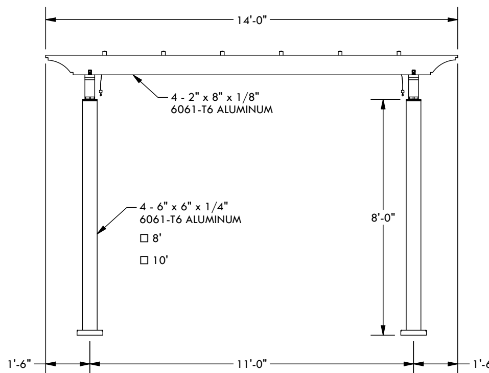
PROJECTION ELEVATION
