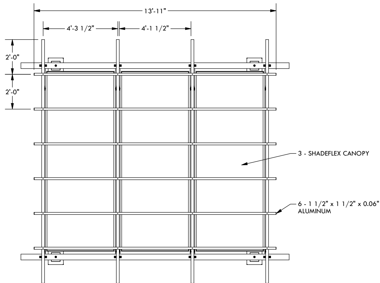
PLAN VIEW
