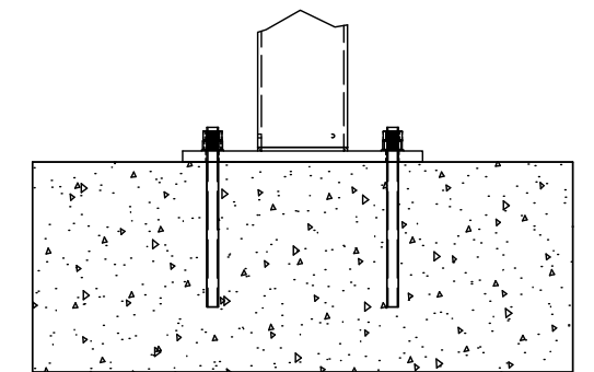
CONCRETE MOUNT
