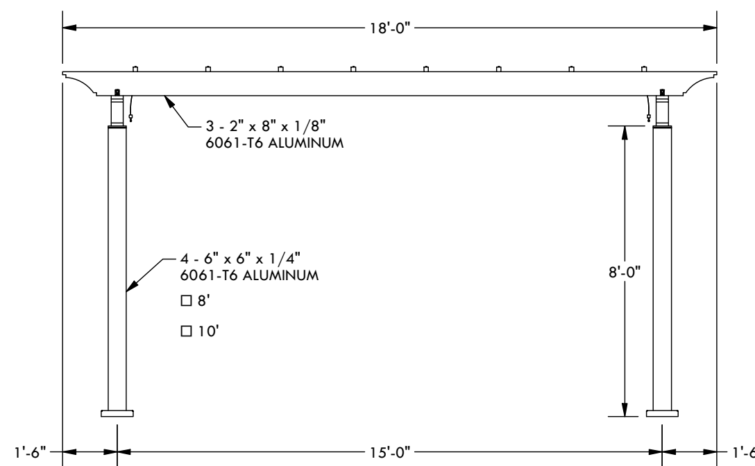
PROJECTION ELEVATION
