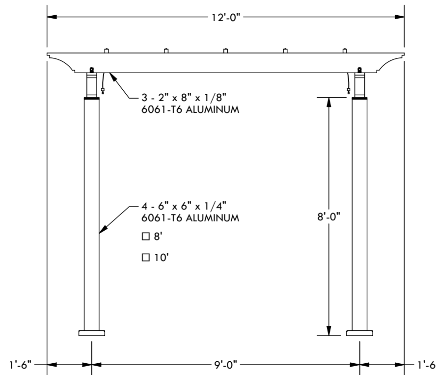
PROJECTION ELEVATION
