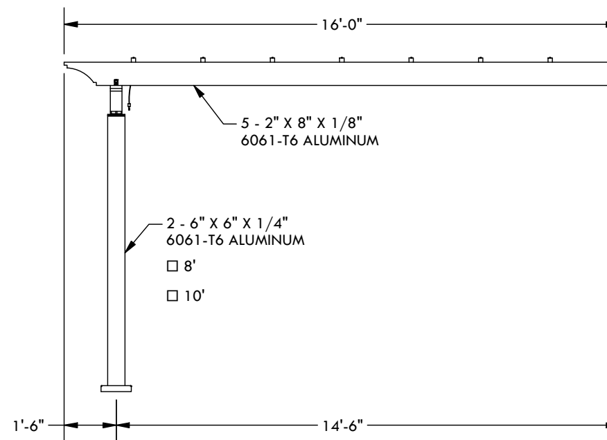
PROJECTION ELEVATION
