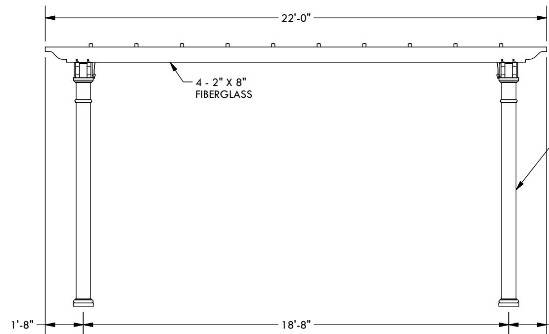
PROJECTION ELEVATION
