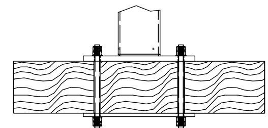
FRAMING MOUNT
