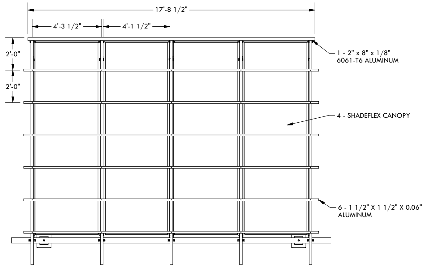
PLAN VIEW
