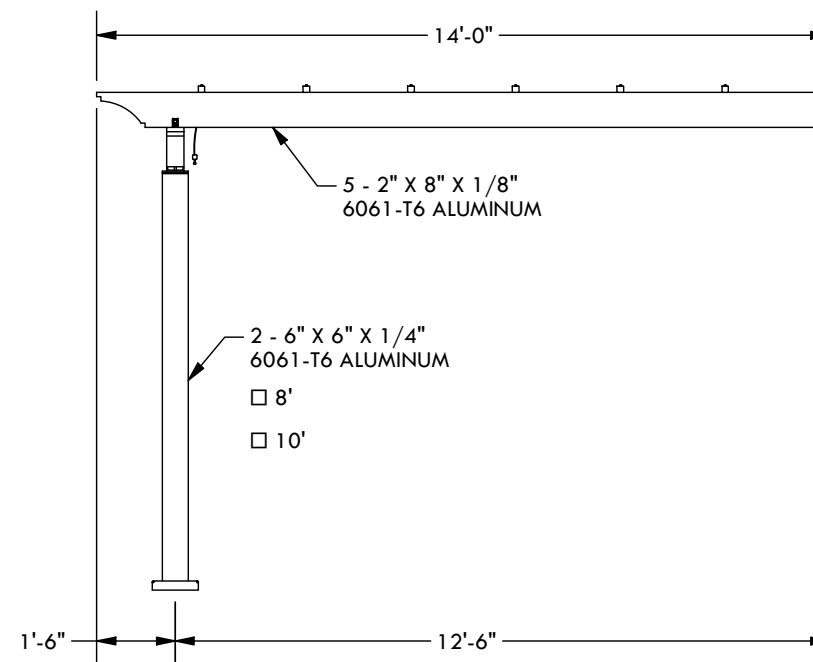
PROJECTION ELEVATION
