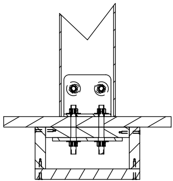
THROUGH BOLT MOUNT
