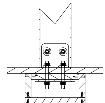
THROUGH BOLT MOUNT
