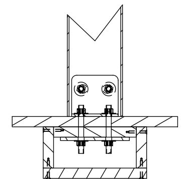
THROUGH BOLT MOUNT
