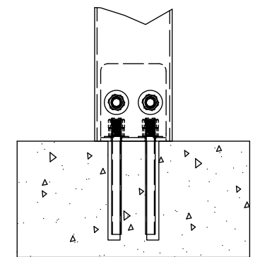
CONCRETE MOUNT
