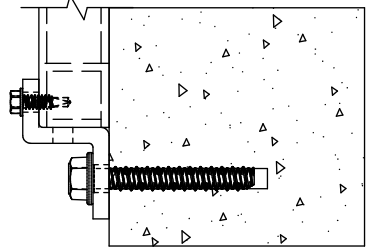
WALL CONNECTION CONCRETE
