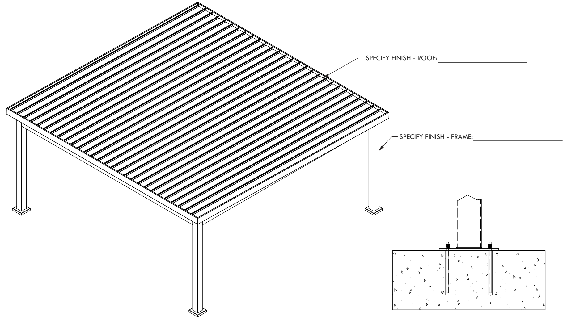
CONCRETE MOUNT
