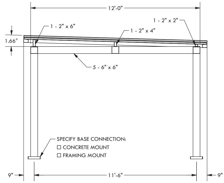
SECTION C-C
