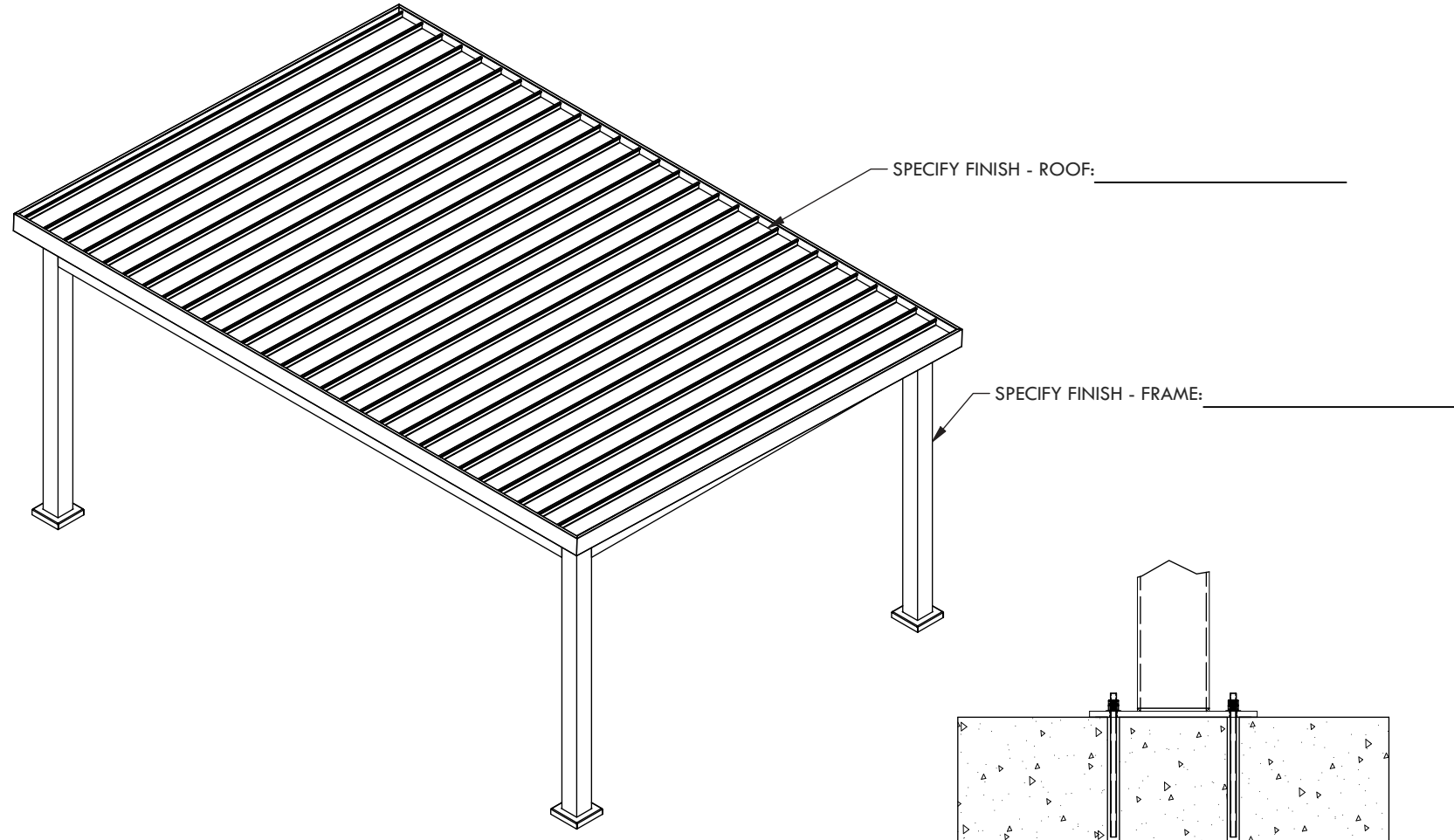
CONCRETE MOUNT
