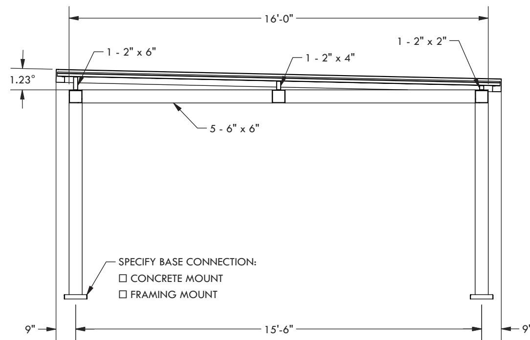
SECTION C-C
