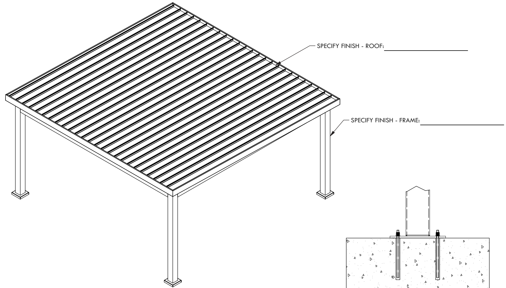
CONCRETE MOUNT
