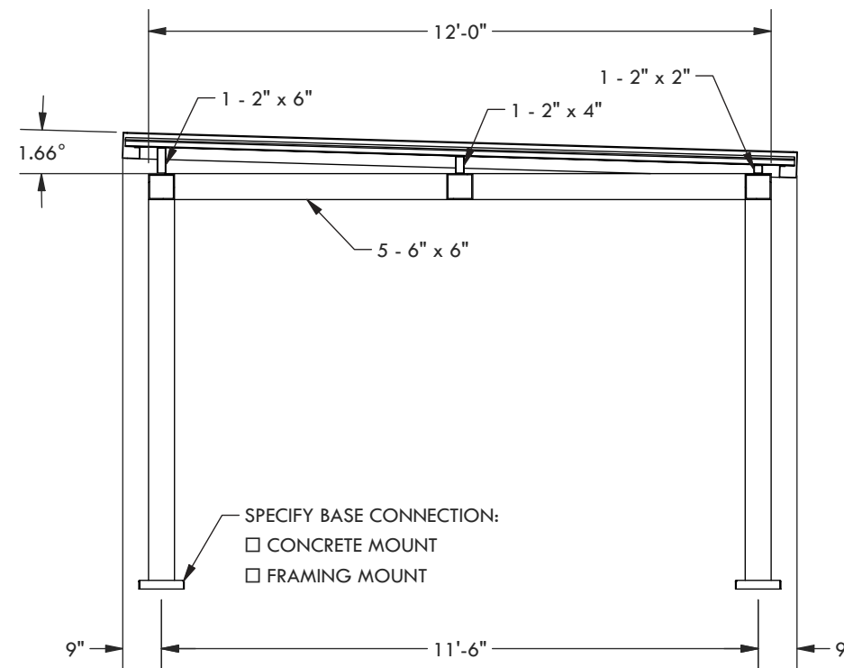
SECTION C-C
