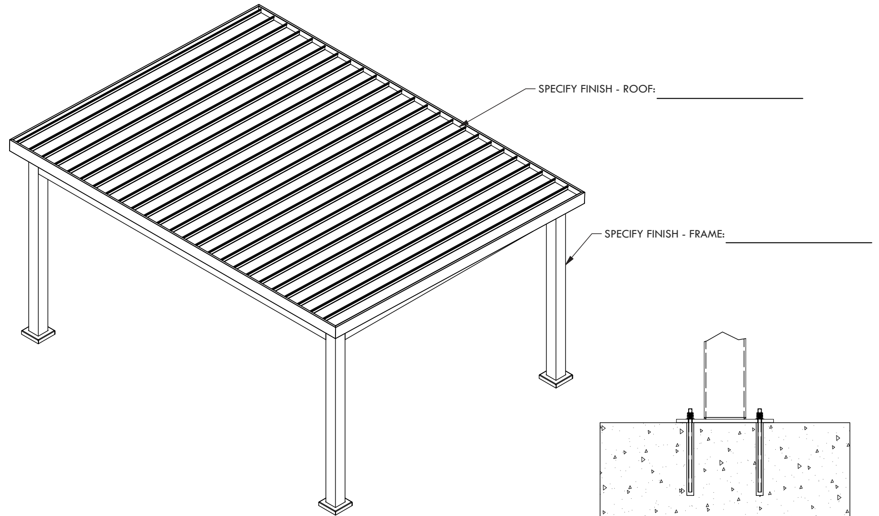
CONCRETE MOUNT
