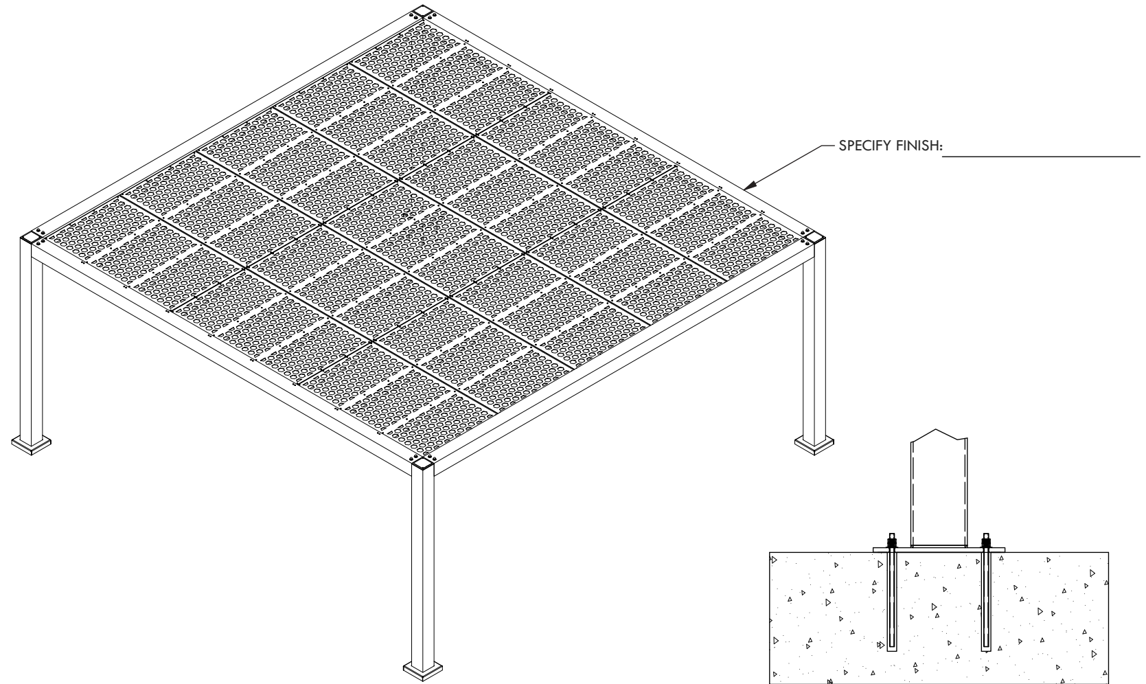
CONCRETE MOUNT
