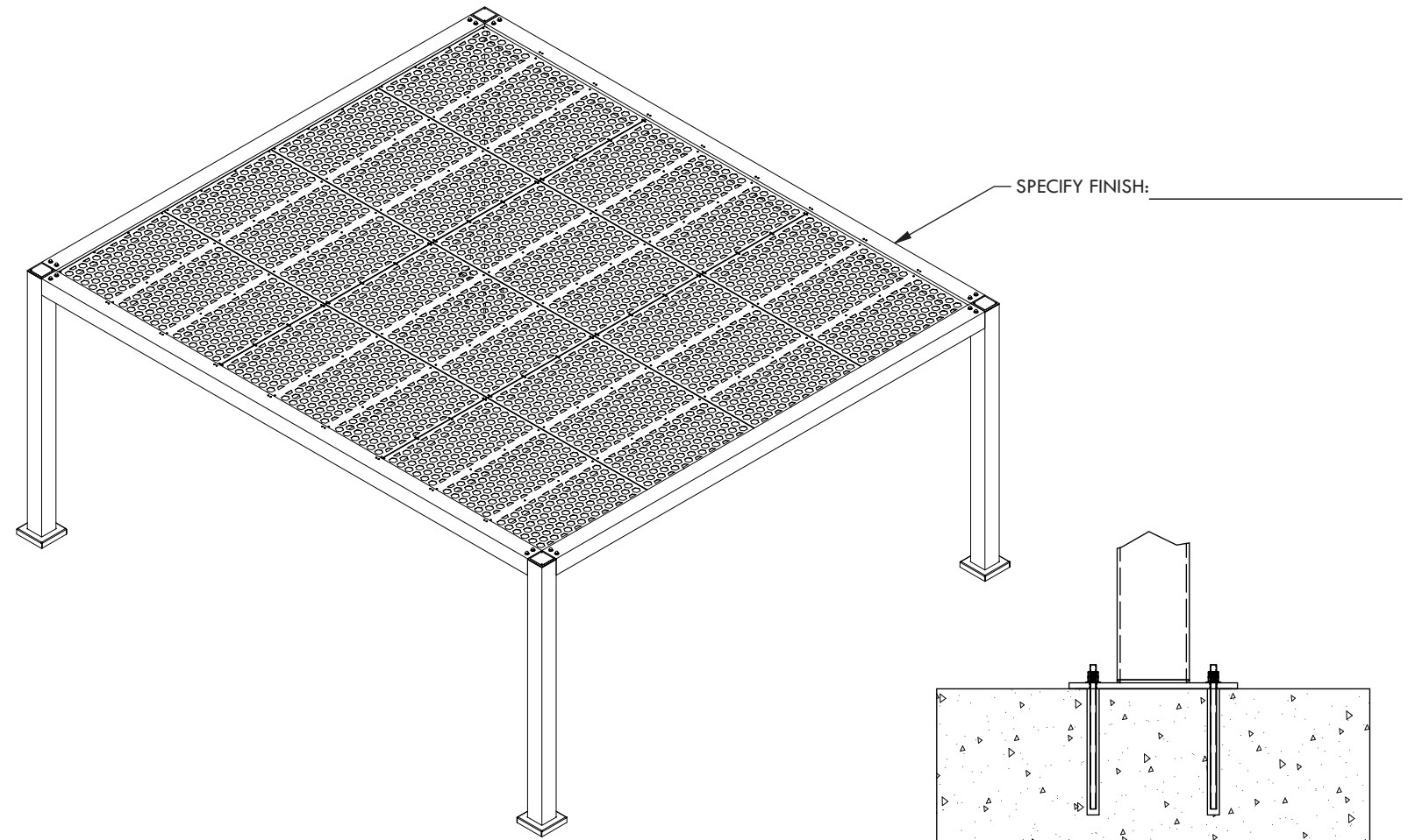
CONCRETE MOUNT
