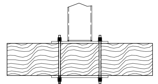
FRAMING MOUNT
