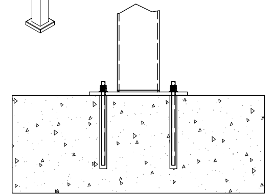
CONCRETE MOUNT
