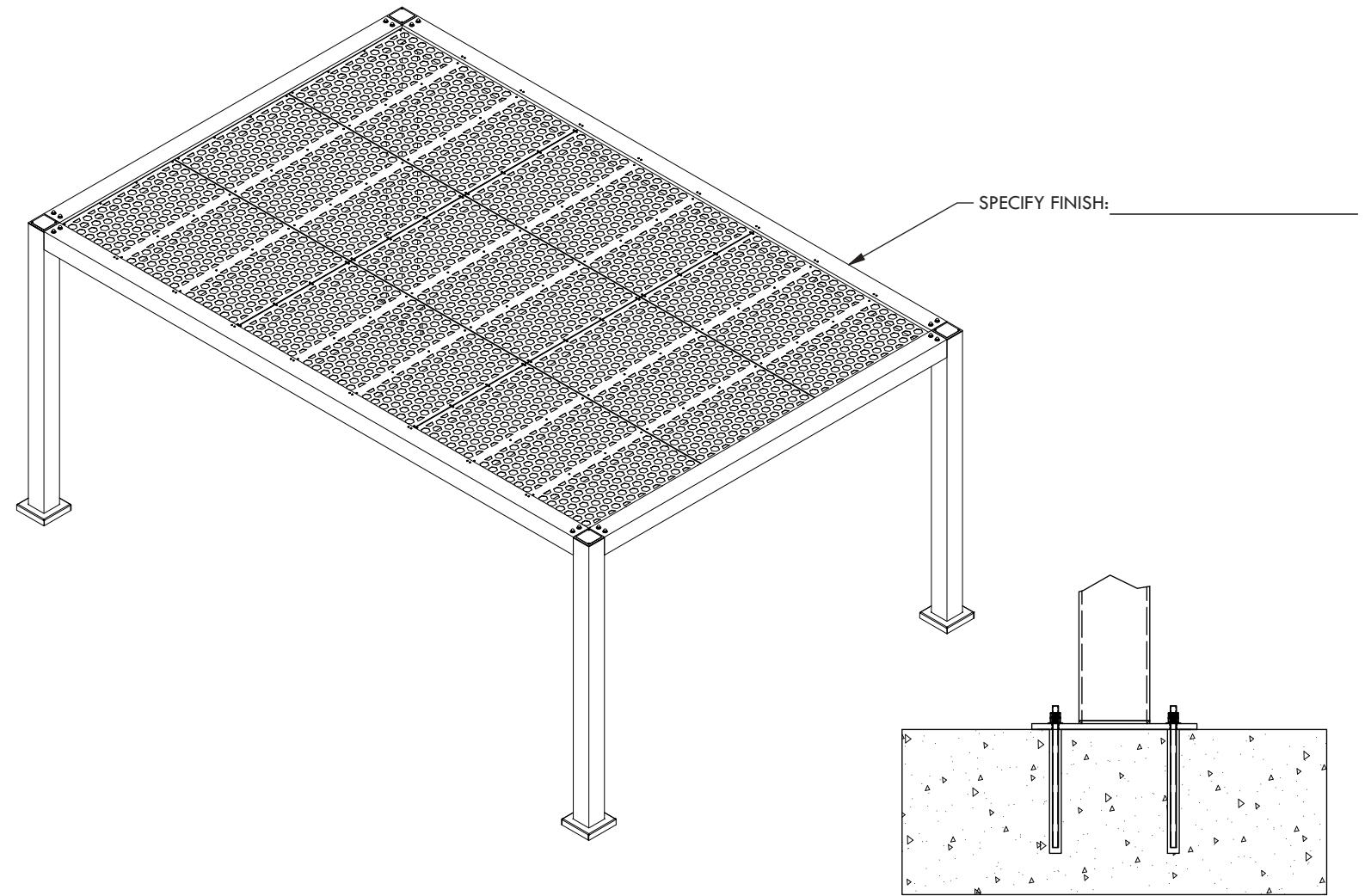
CONCRETE MOUNT
