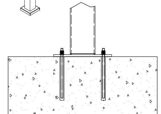
CONCRETE MOUNT
