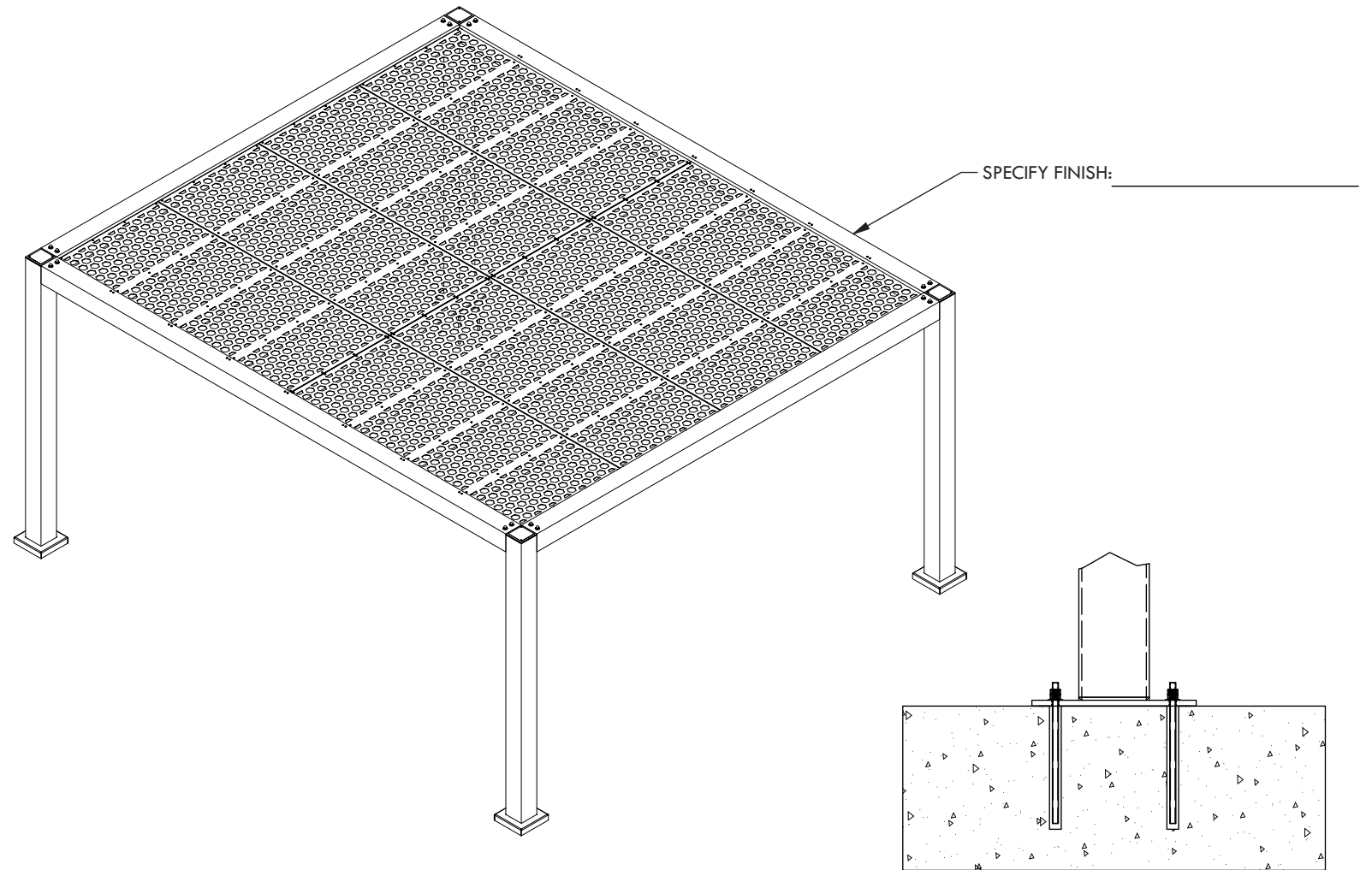
CONCRETE MOUNT
