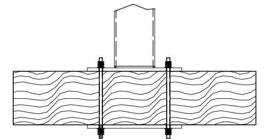
FRAMING MOUNT
