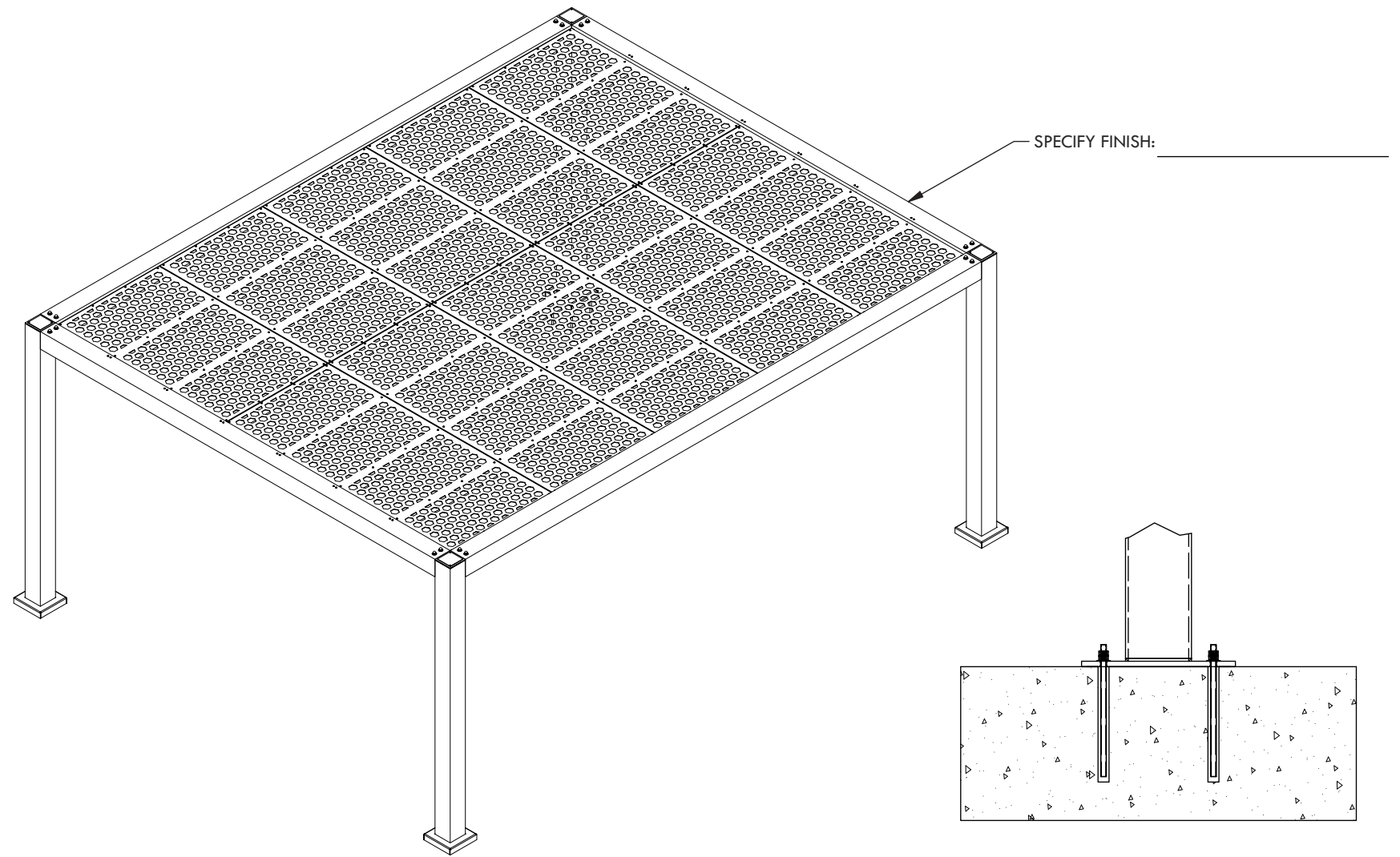
CONCRETE MOUNT
