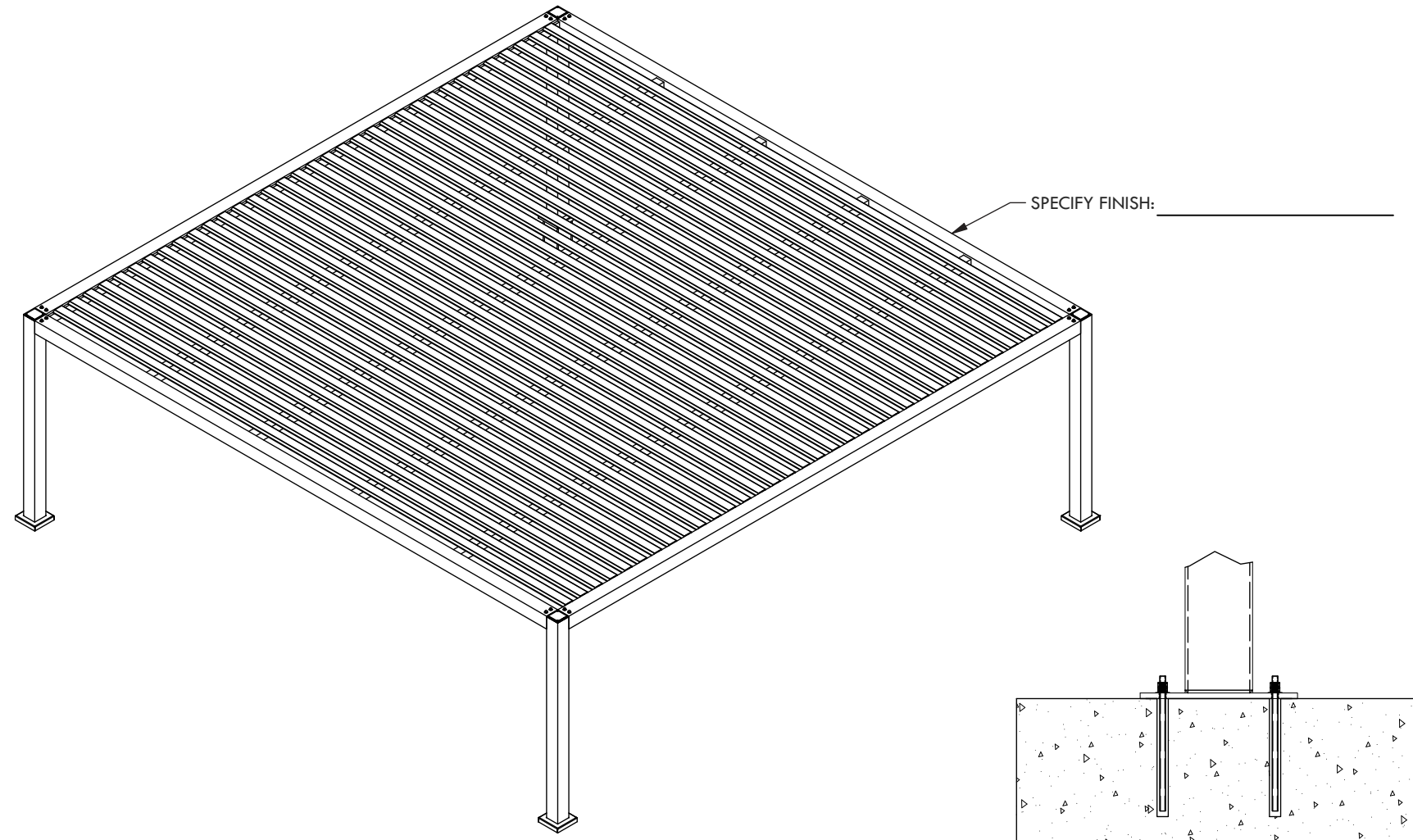
CONCRETE MOUNT
