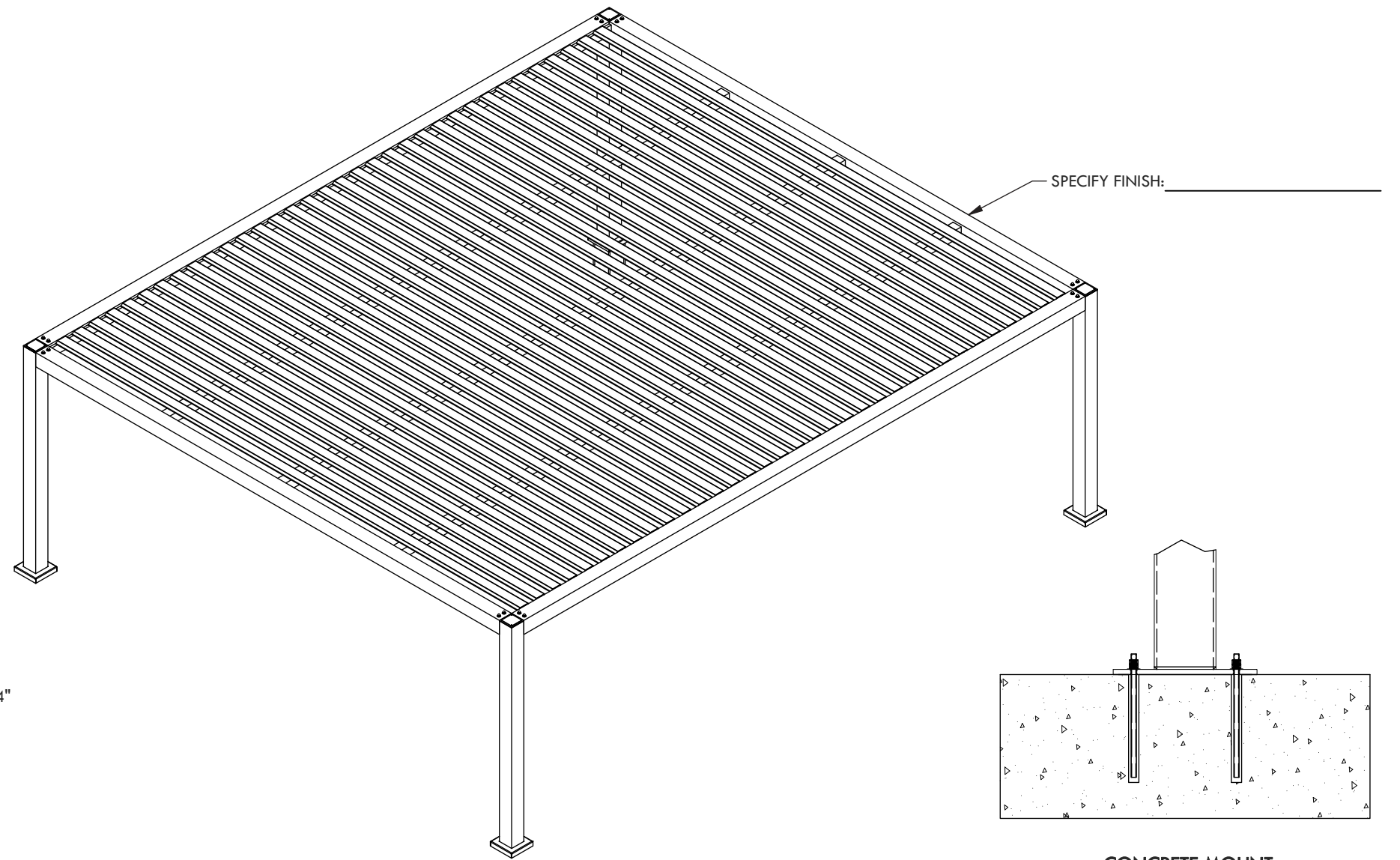
CONCRETE MOUNT
