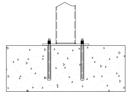
CONCRETE MOUNT
