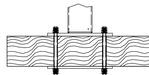
FRAMING MOUNT
