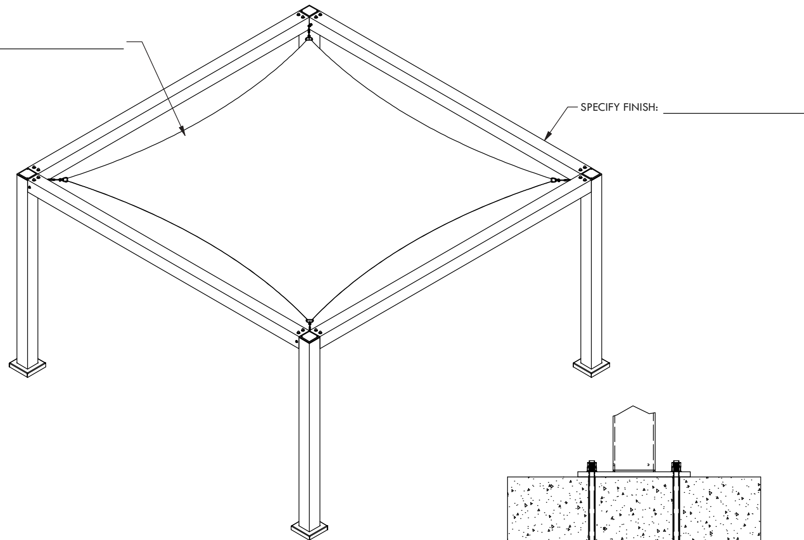
CONCRETE MOUNT
